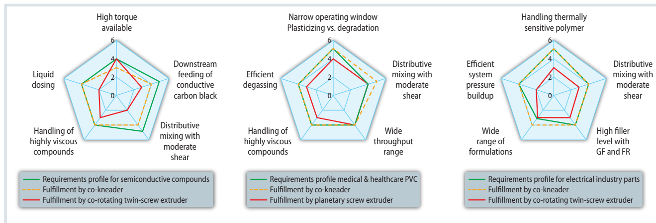
Fig. 6. Technology comparison: degree of fulfillment of requirements for manufacturing a) semiconductive compounds for high-voltage cables, b) PVC compounds for medical technology, and c) parts for the electrical industry, each in comparison with a competing compounding technology; GF = glass fibers, FR = flame retardants [5] Source: Buss; graphic: © Hanser
