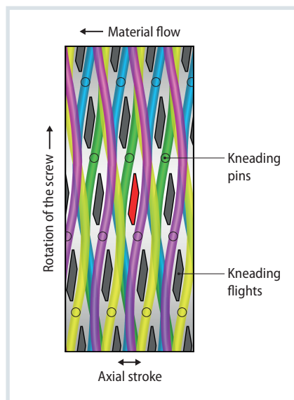
Fig. 5. Mixing effect of a four-flight screw element spread out in the plane and abstractly represented using the kneading pin paths that arise during one complete revolution of the screw shaft. The plastic mass is sheared, split, and refolded between the kneading pins and the kneader flights passing them in real operation Source: Buss; graphic: © Hanser
