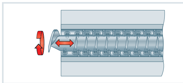
Fig. 4. Interaction between screw shaft rotation and reciprocation Source: Buss; graphic: © Hanser
